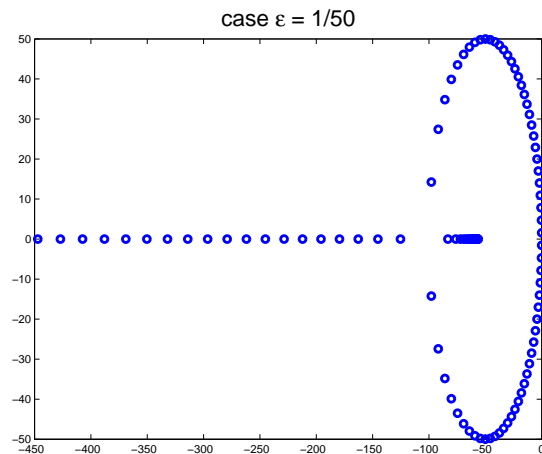
Fig. 1. Spectrum with structural damping.
