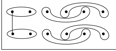
Figure 5: a class with three degrees of freedom
