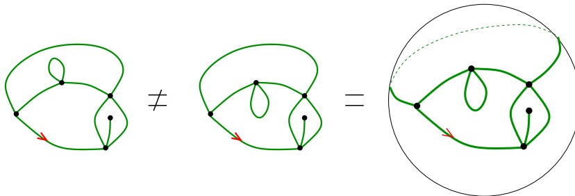
Figure 1: Two distinct planar maps, and a spherical representation of the second.
