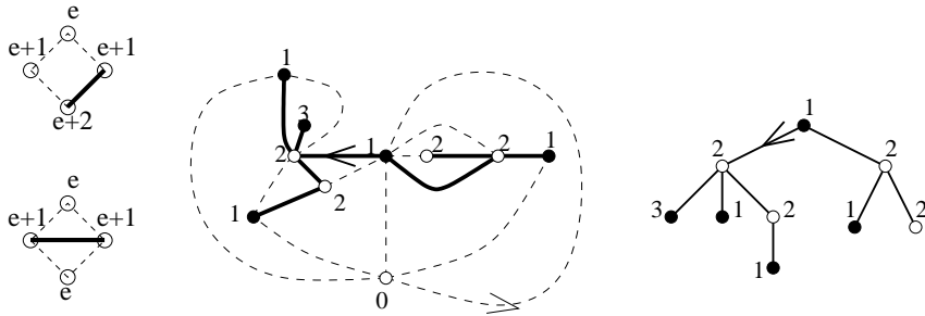
Figure 5: The rules of selection of edges and an example.
