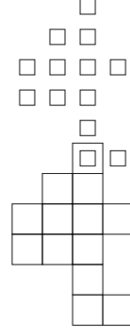
FIGURE 4. \vec{T}_5(\mathcal{C}) \cap \vec{T}_{11}(\mathcal{C}) is a unit square
