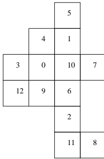
FIGURE 2. abcaababcabca is a roundwalk of \mathcal{C}
