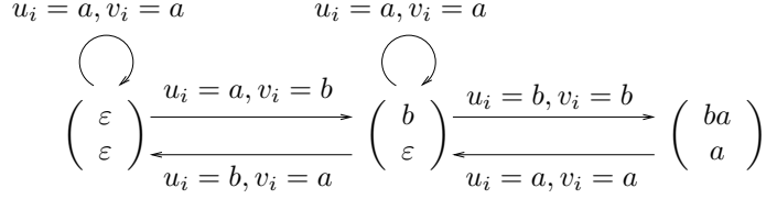
FIGURE 1. Potential balanced pairs produced by the action of \sigma on (u, v) for the Fibonacci case
